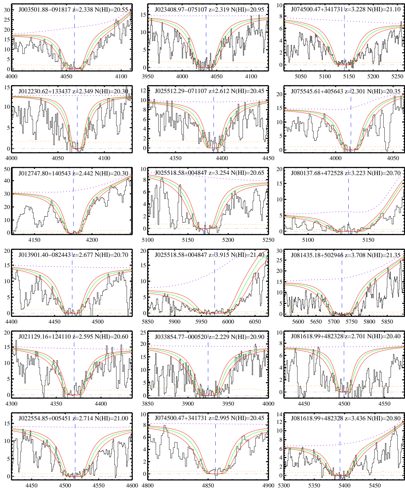
FIG. 1.— Ly \alpha profiles of the 71 damped Ly \alpha systems comprising the full statistical sample from the SDSS Data Release 1. The dotted line traces the assumed continuum of the quasar and the green solid line is a Voigt profile corresponding to the N(\text{HI}) values given in Table 2. All plots have angstroms along the x-axis and flux ( f_{\lambda} \times 10^{17} cgs) along the y-axis.
